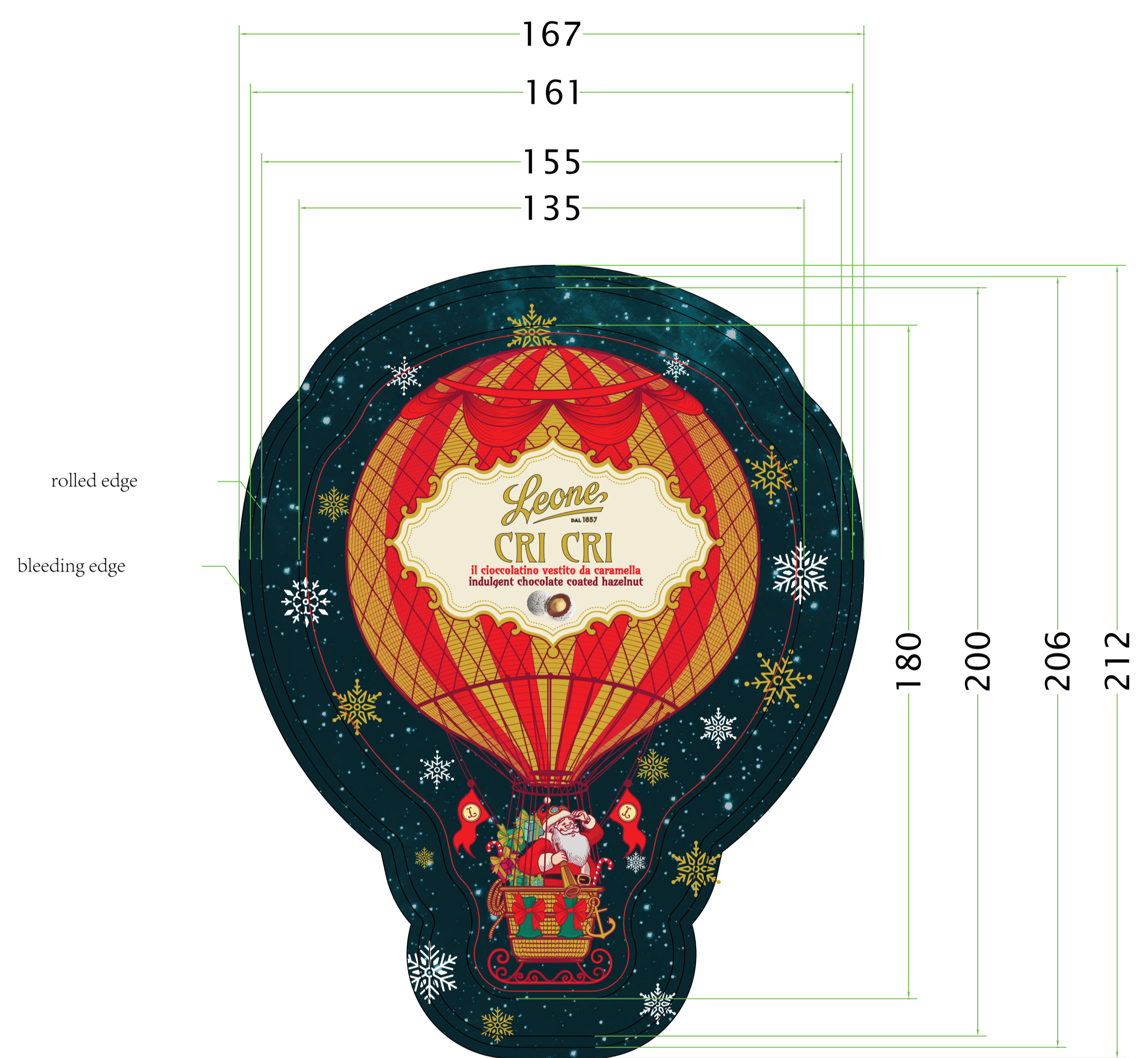
layout drawing of lid
